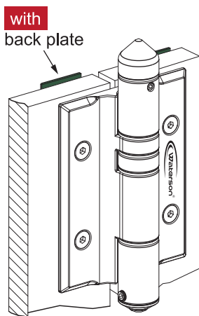
K51P Full Surface Clamping Style
